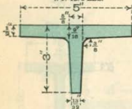
T. 169 WT. 13.6 LBS.
