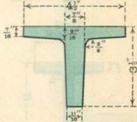
T. 84 WT. 9.3 LBS.
