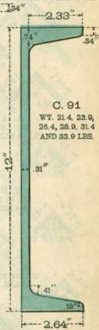
SPECIAL 12" CHANNEL.
