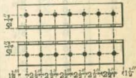
4" x 4" x \frac{3}{8} " ANGLE - 18" LONG
