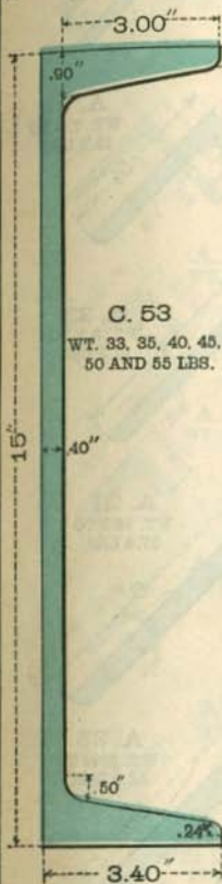
STANDARD 15" CHANNEL.
