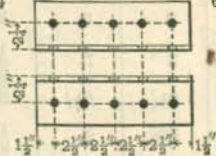
4" x 4" x \frac{3}{8} " ANGLE - 13" LONG
