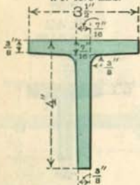
T. 65 WT. 7.2 LBS.
