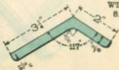
A. 61 WTS. 1.3 AND 1.8 LBS.
