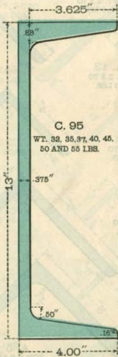
SPECIAL 13" CHANNEL.
