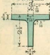
T. 65 WT. 7.2 LBS.
