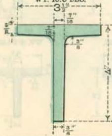
T. 101 WT. 10.0 LBS.
