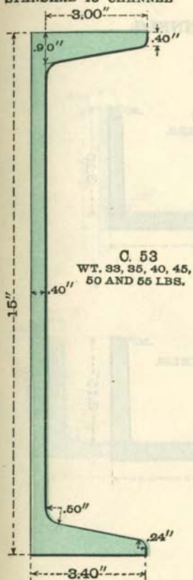
STANDARD 15" CHANNEL
