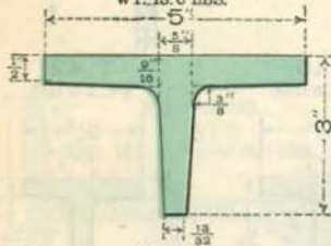
T. 101 WT. 10.0 LBS.
