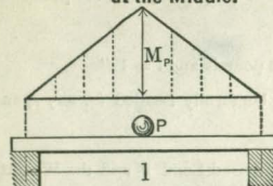
Diagram for Superimposed Load:— Draw triangle having M_p = \frac{Pl}{4} Diagram for Dead Load similar to Case(1)
