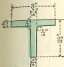
T. 27 WT. 4.5 LBS.
