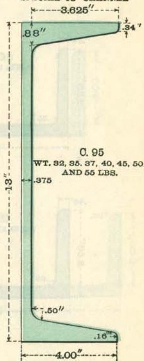
SPECIAL 13" CHANNEL
