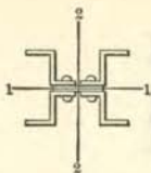
Z-Bar Columns.
