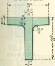
T. 67 WT. 6.8 LBS.
