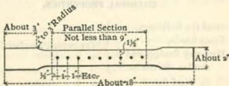
Piece to be the same thickness as the plate.
