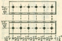
4" x 4" x 3/8" ANGLE - 15" LONG
