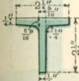
T. 41 WT. 4.2 LBS.
