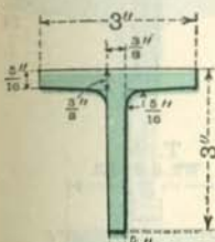
T. 41 WT. 4.2 LBS.
