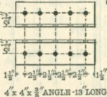
FOR 18" BEAMS
