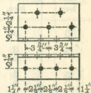
6" x 4" x 3/8" ANGLE - 10" LONG
