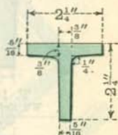
T. 37 WT. 3.7 LBS.
