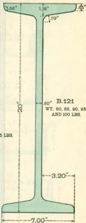
SPECIAL 20" BEAM.
