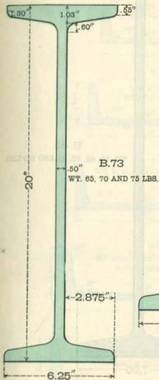
STANDARD 20" BEAM.
