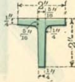
T. 37 WT. 3.7 LBS.
