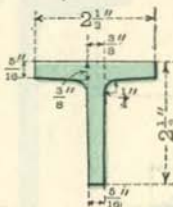
T. 39 WT. 4.4 LBS.
