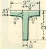
T. 39 WT. 4.4 LBS.
