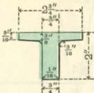
T. 62 WT. 7.5 LBS.
