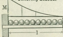
Diagram for Total Load:— Draw Parabola having M = \frac{Wl^2}{2}
