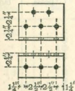
6" x 4" x 3/8" ANGLE - 7 1/2" LONG
