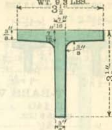
T. 97 WT. 9.3 LBS.
