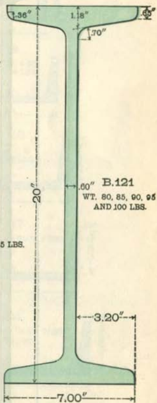
SPECIAL 20" BEAM.
