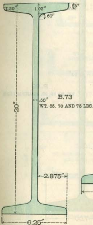
STANDARD 20" BEAM.
