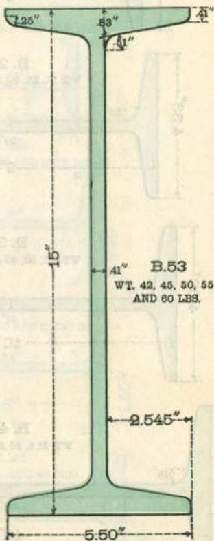
STANDARD 15" BEAM.
