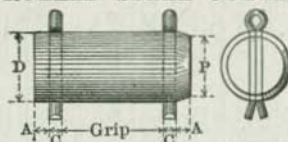
Dimensions of Pin in Inches.
