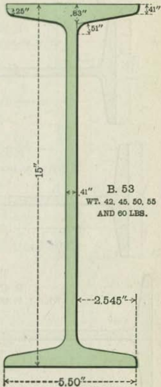
STANDARD 15" BEAM.
