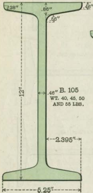
SPECIAL 12" BEAM.
