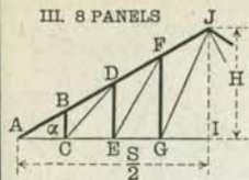
III—8 Panels.
