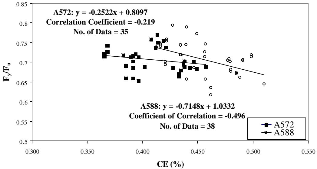
Figure 3.3: CE versus Yield to Tensile Ratio for the 4-Mill Group.
